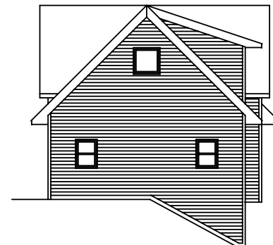
WEST ELEVATION
