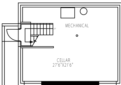
BASEMENT FLOOR PLAN
