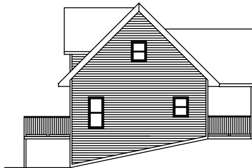
EAST ELEVATION
